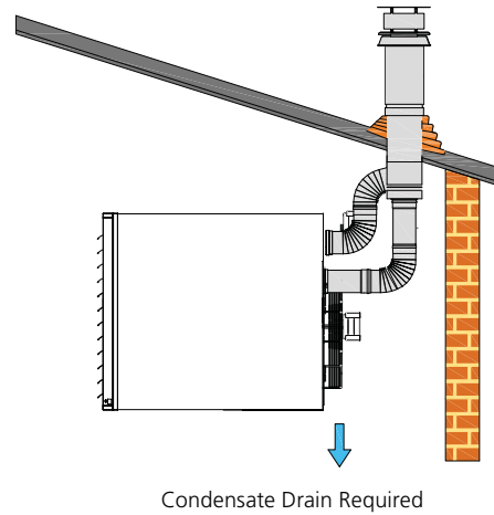
Balanced flue roof outlet (type C32)
